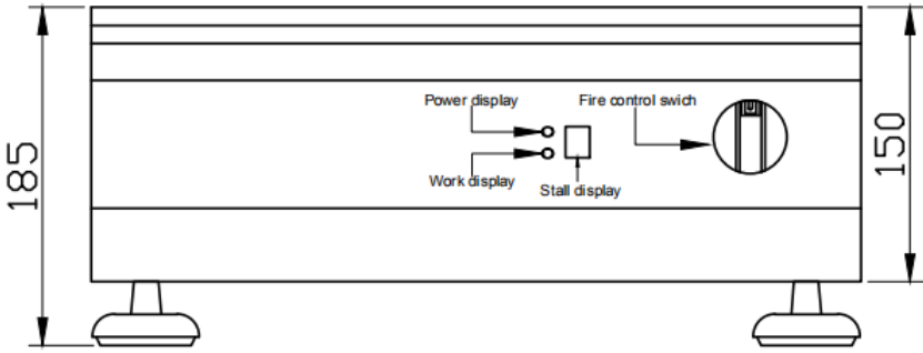
Vista Frontal
